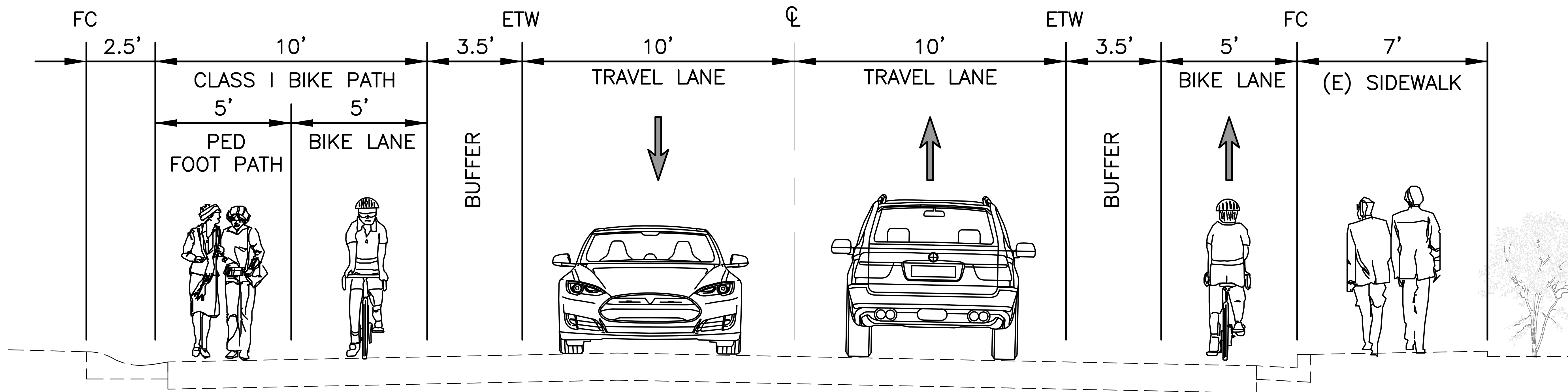
CONCEPT 3 PROPOSED CROSS SECTION - FACING EAST JARDIN DRIVE
