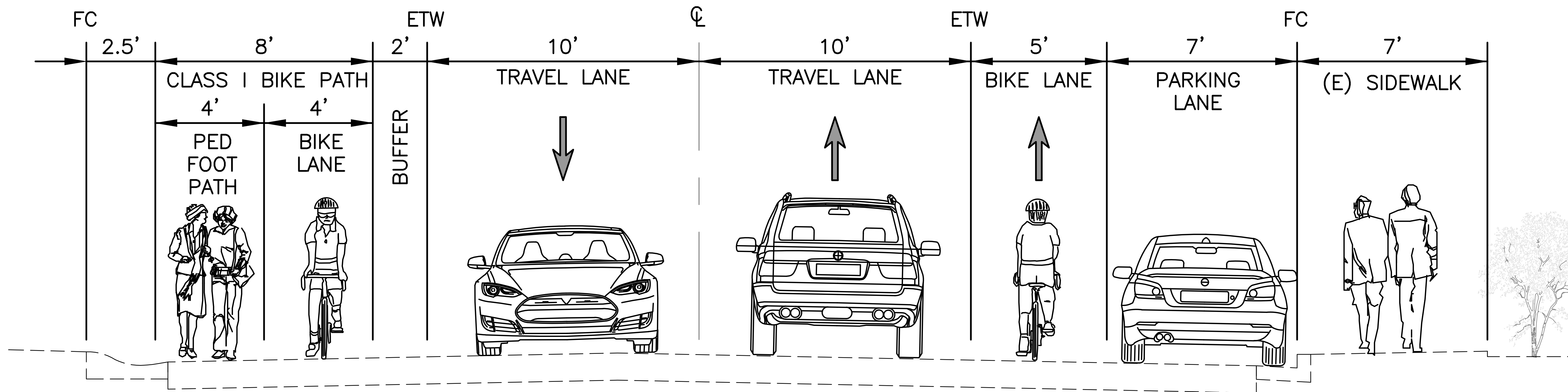
CONCEPT 2 PROPOSED CROSS SECTION - FACING EAST JARDIN DRIVE
