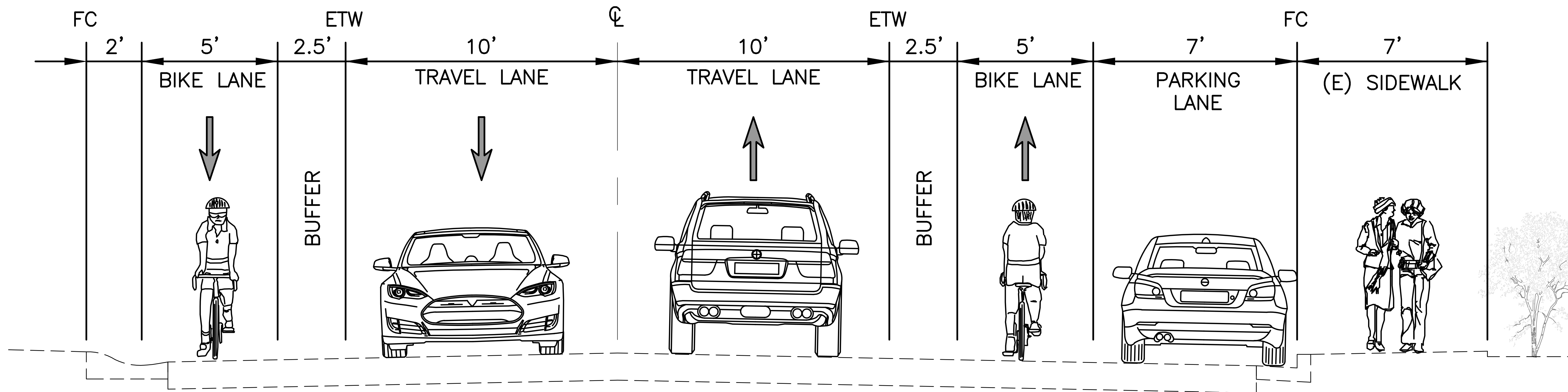
CONCEPT 1 PROPOSED CROSS SECTION - FACING EAST JARDIN DRIVE
