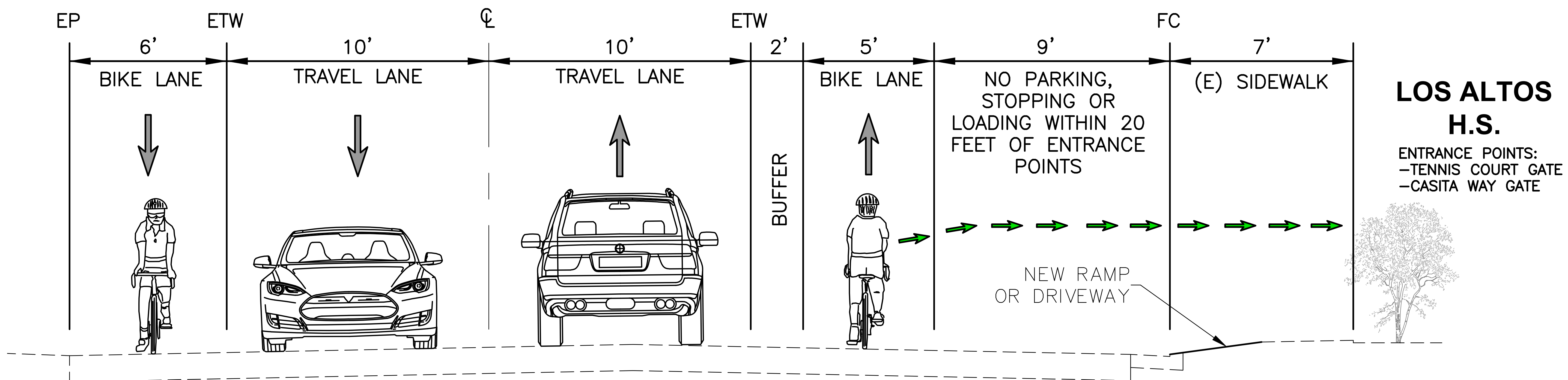
RECOMMENDED PLAN JARDIN DRIVE PROPOSED CROSS SECTION - FACING EAST AT STUDENT ENTRANCE POINTS TO HIGH SCHOOL
