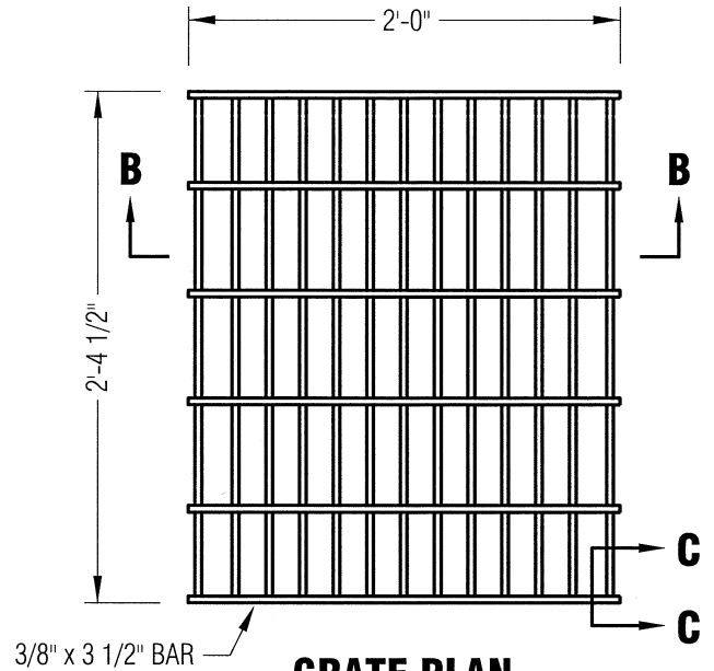
GRATE PLAN
