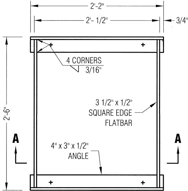
FRAME PLAN
