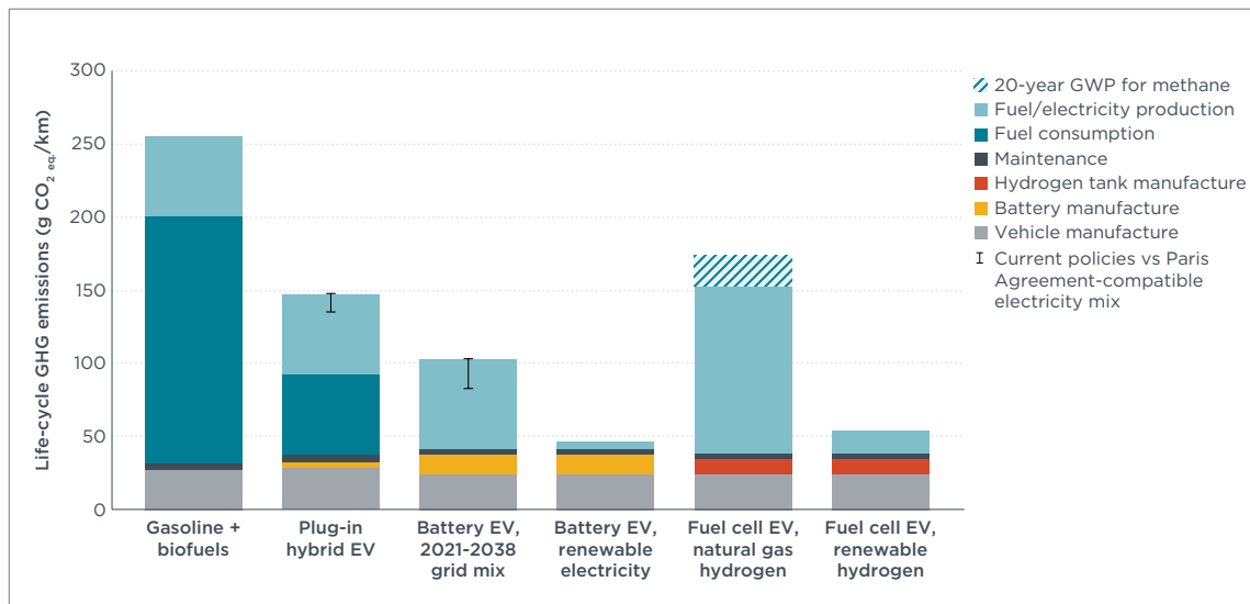
Figure 18 Life-cycle GHG emissions of passenger car segment gasoline ICEVs, PHEVs, BEVs, and FCEVs registered in the United States in 2021.
