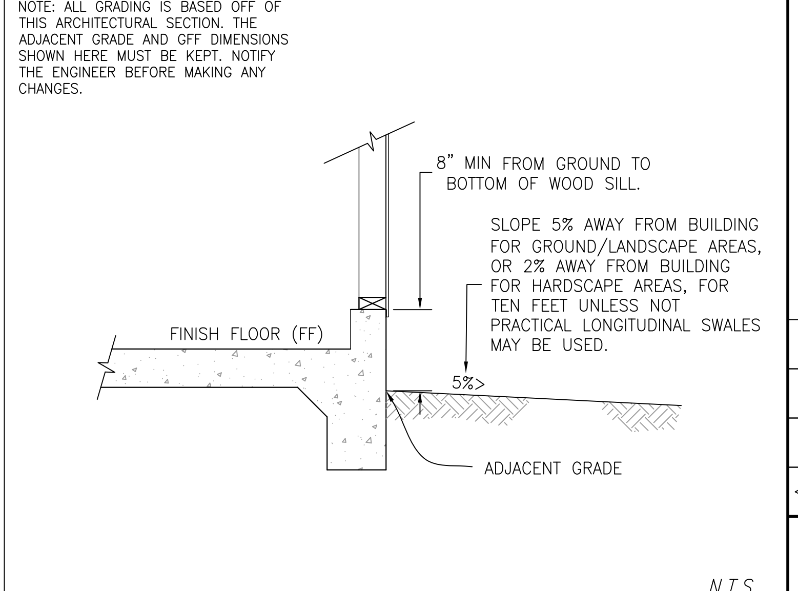
D TYPICAL FOUNDATION/GFF/GROUND SECTION
