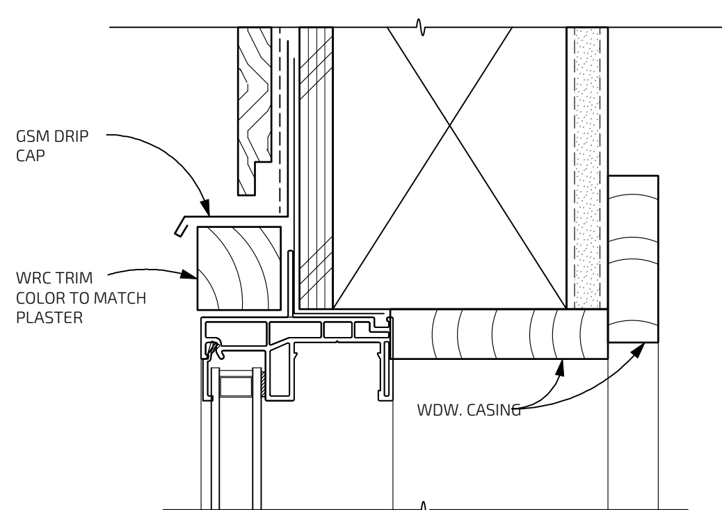
TYP. WDW. JAMB DETAIL @ CEMENT PLASTER FINISH 11
