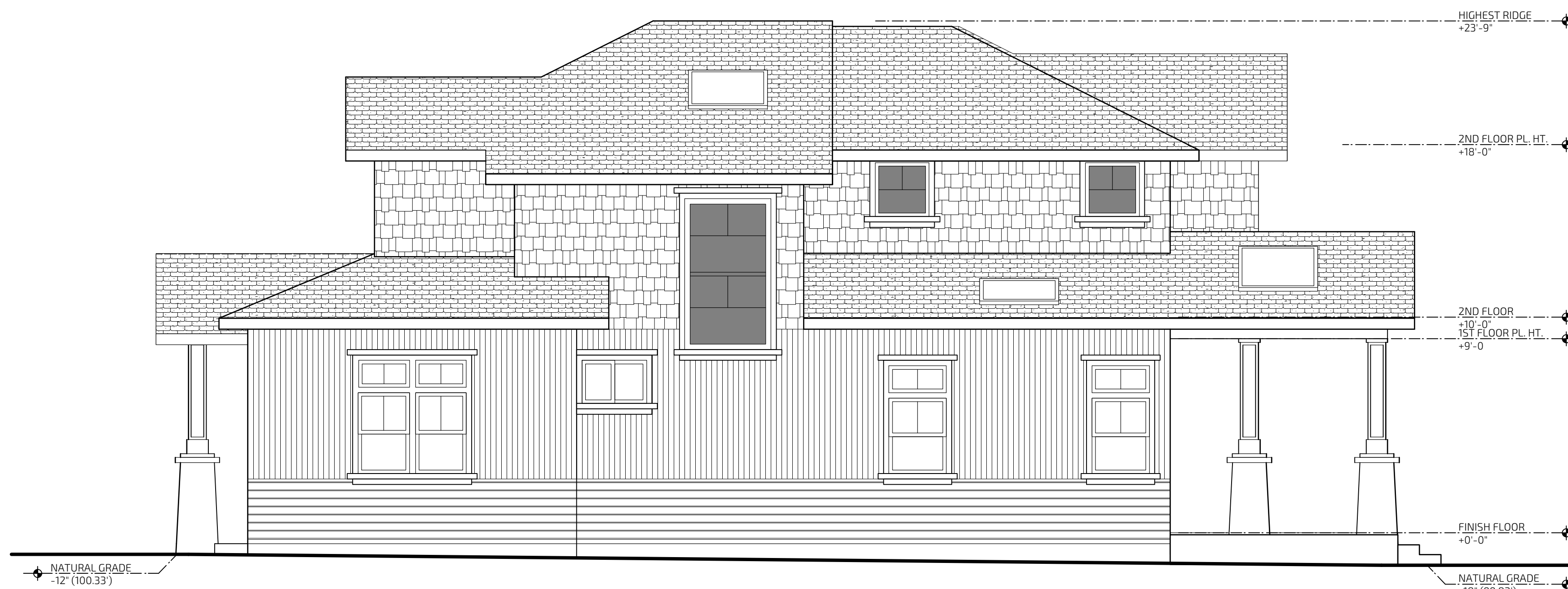
0' 2.5' 5' 7.5' 10' 12.5' 15' PROPOSED WEST (RIGHT) ELEVATION 2 SCALE 1/4" = 1'-0"
