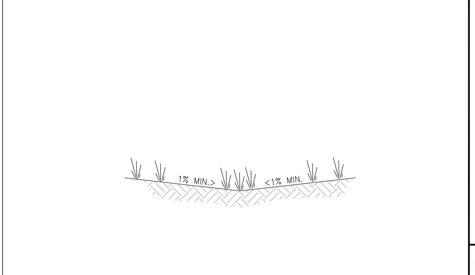
G EARTHEN SWALE DETAIL
