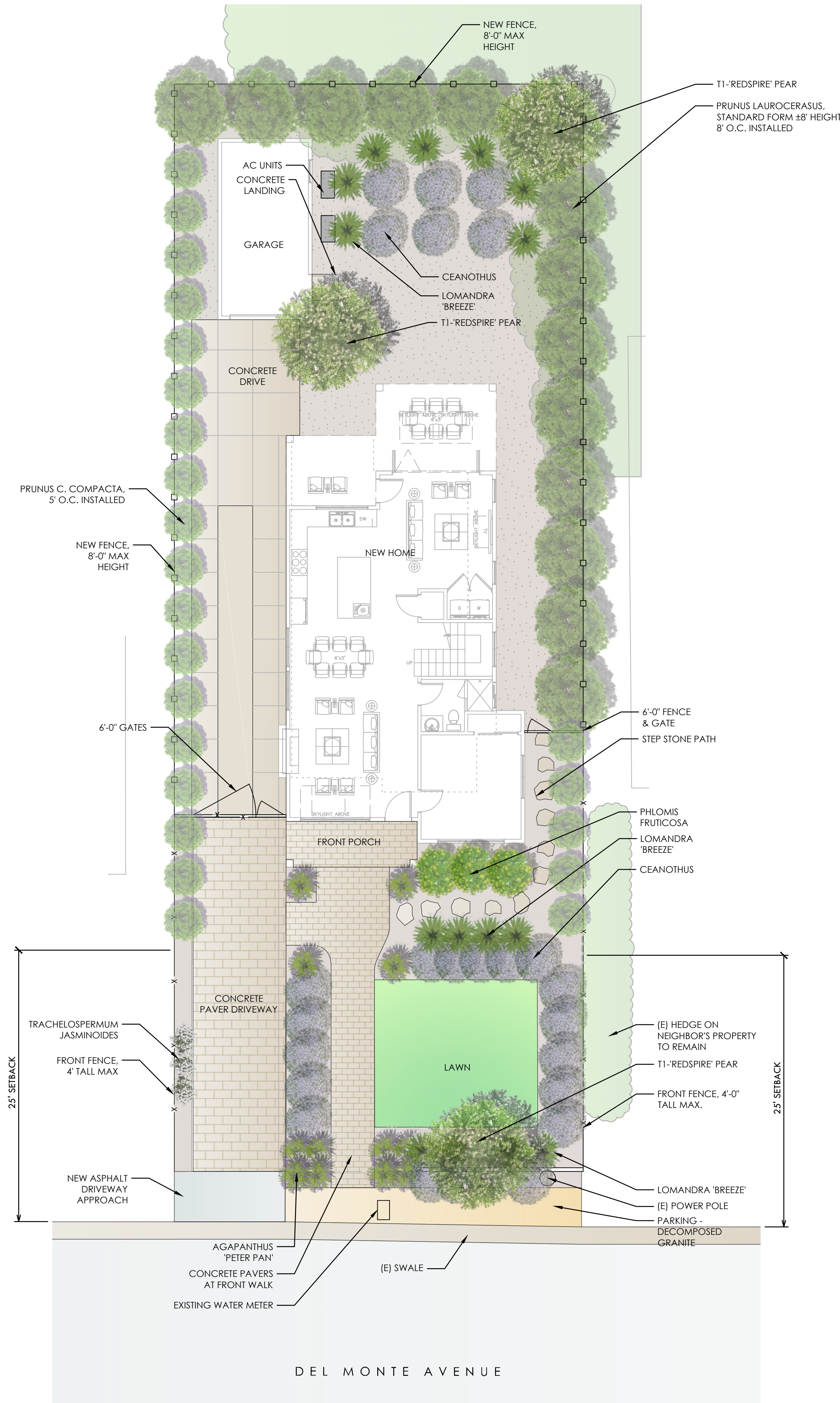
ILLUSTRATIVE SITE PLAN
