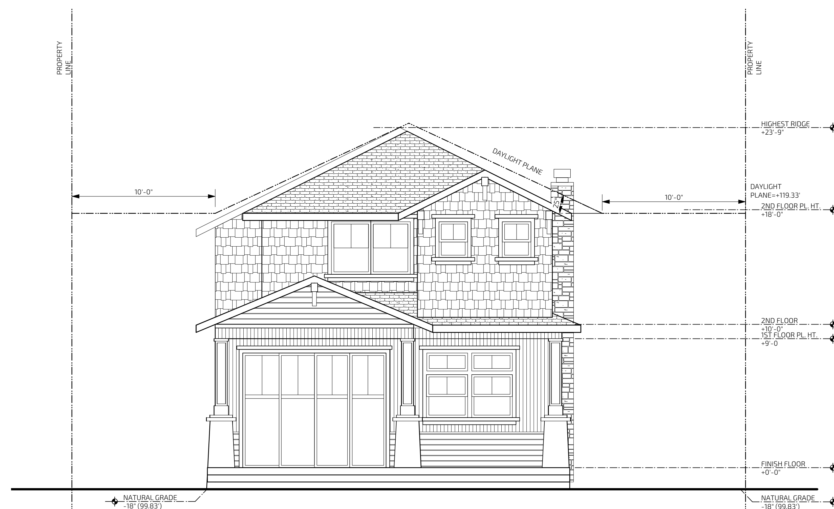
0' 2.5' 5' 7.5' 10' 12.5' 15' PROPOSED SOUTH (BACK) ELEVATION 1 SCALE 1/4" = 1'-0"
