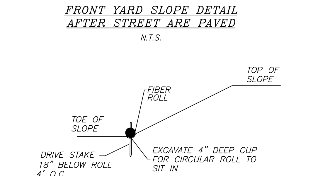
FIBER ROLL INSTALLATION DETAIL N.T.S.
