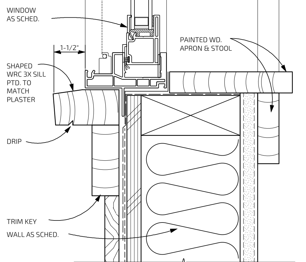
TYPICAL WDW. SILL, MEETING RAIL & HEAD DETAILS @ CEM. PLASTER FINISH (DR HEAD SIM.) 10
