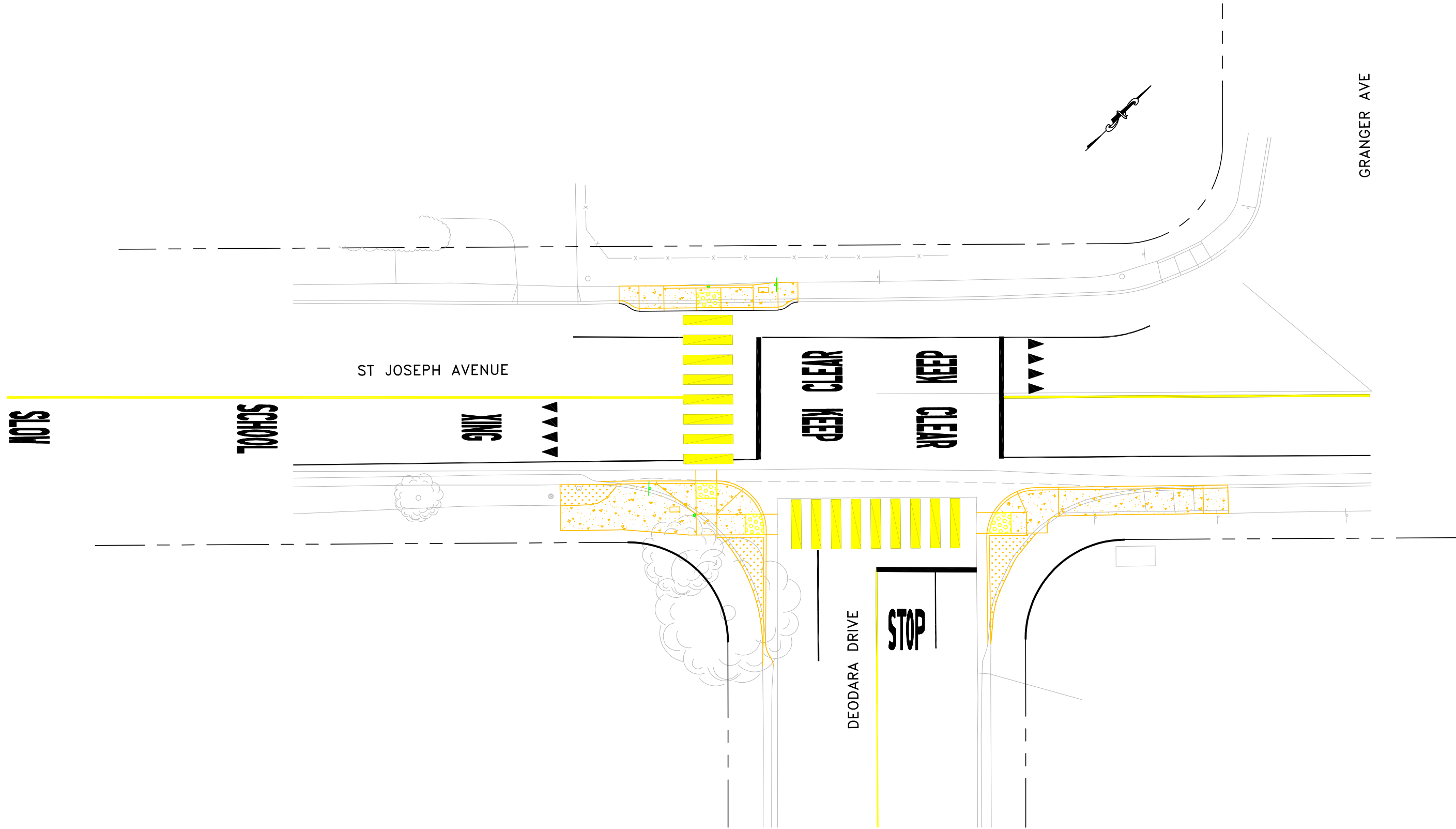
① LOCATION #6 - DEODARA DR AND ST. JOSEPH AVE IMPROVEMENT PLAN SCALE: 1"=10'
