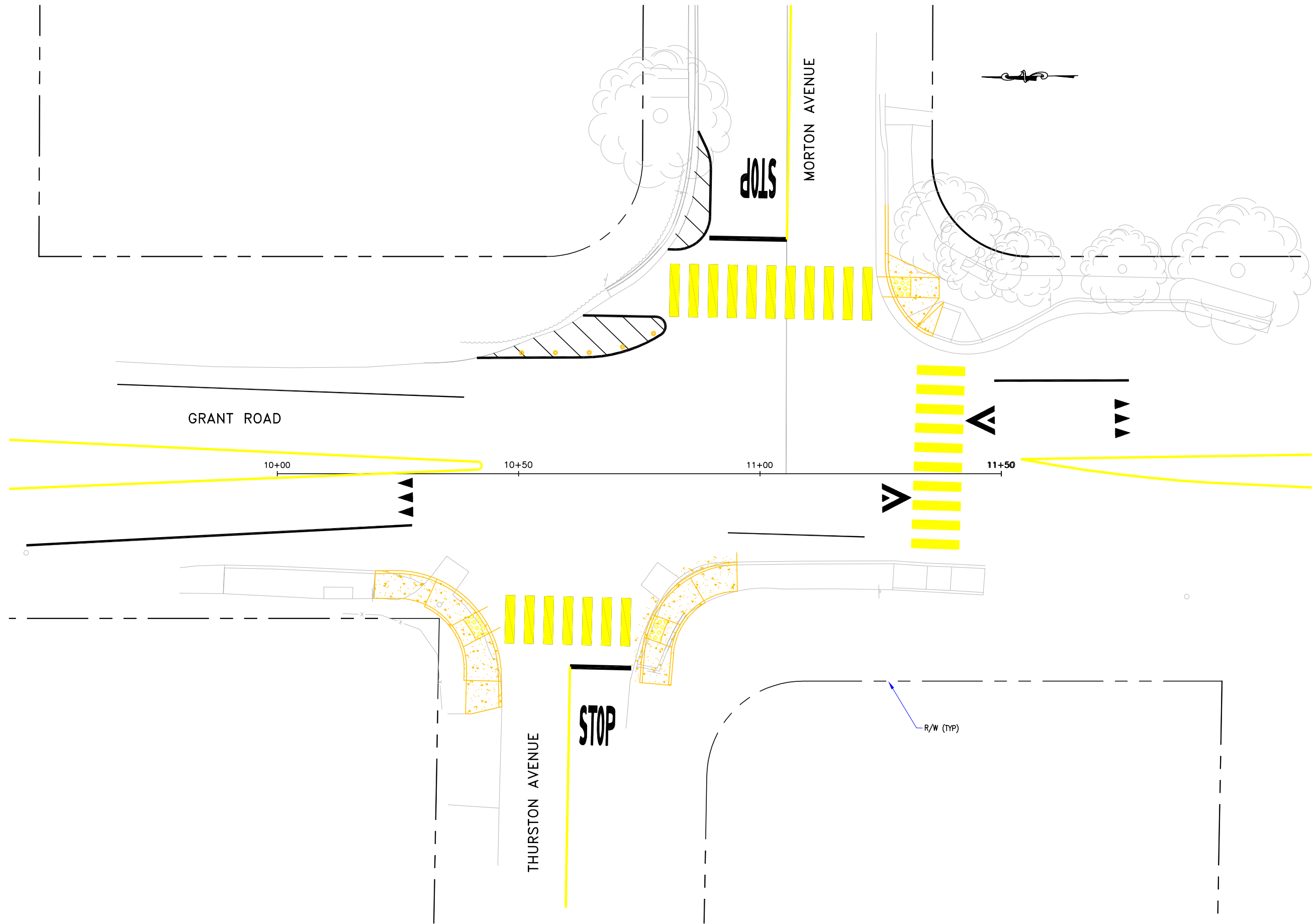
1 LOCATION #5 - GRANT RD, THURSTON AVE, AND MORTON AVE IMPROVEMENT PLAN SCALE: 1"=10'
