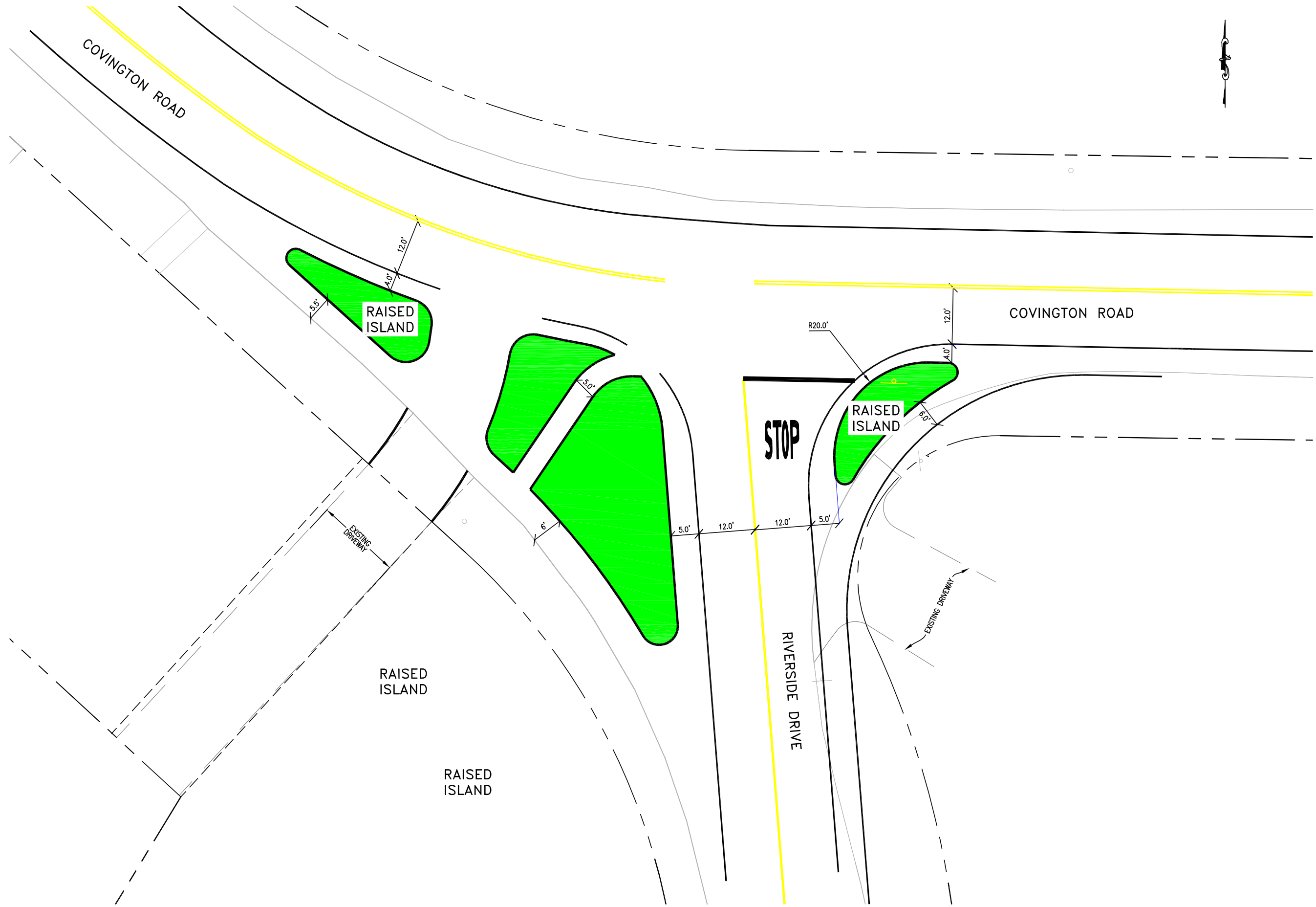
① LOCATION #3 - COVINGTON RD AND RIVERSIDE DR IMPROVEMENT PLAN SCALE: 1"=10'
