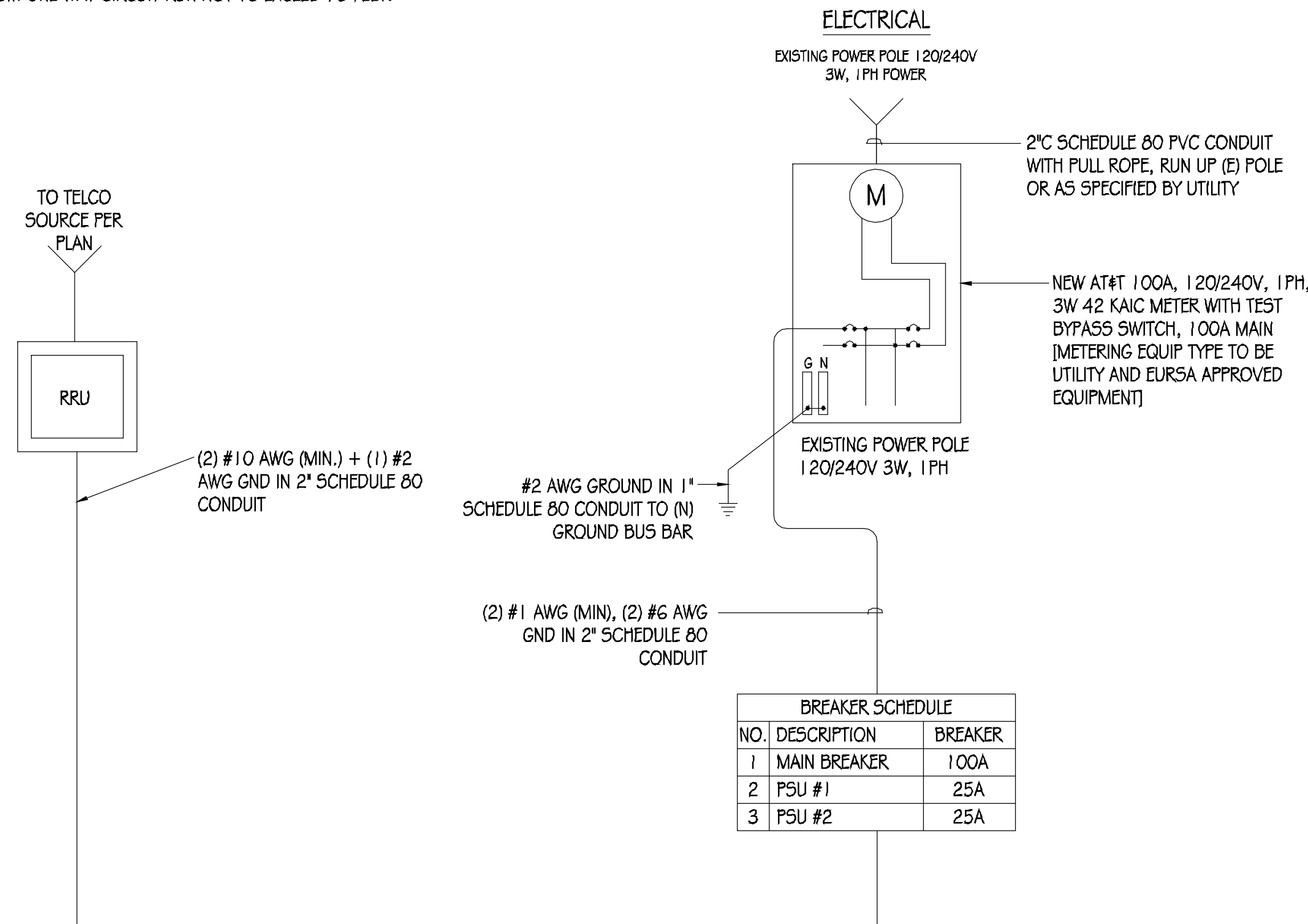
SINGLE-LINE DIAGRAM
