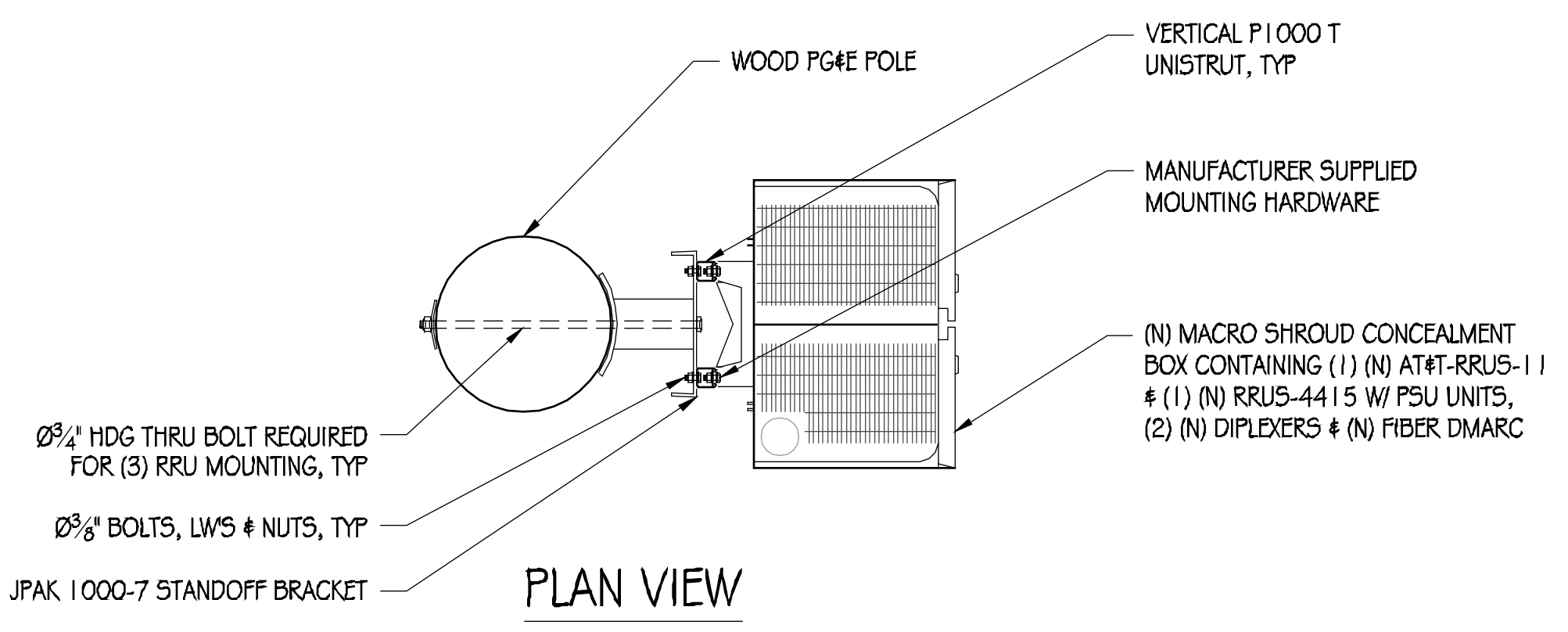
3 RRU MOUNTING DETAIL 1" = 1'
