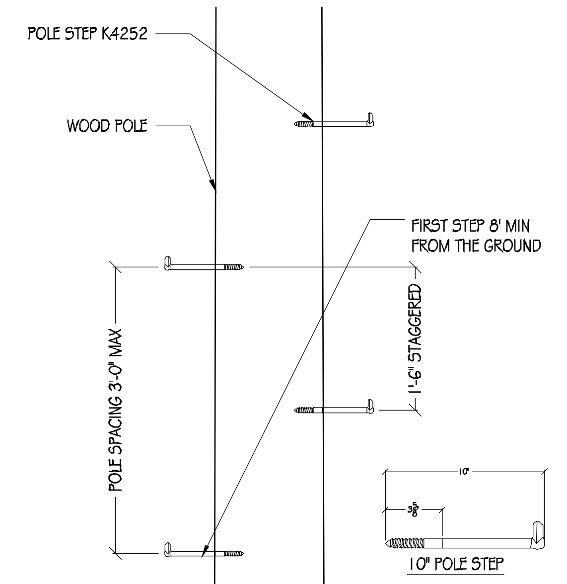
5 POLE STEP 1" = 1'
