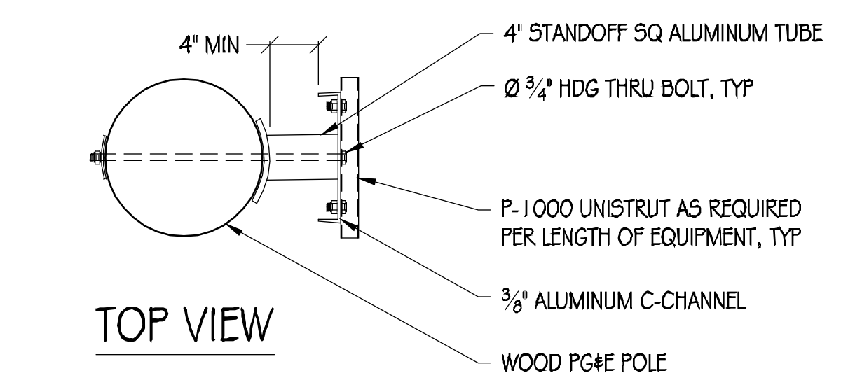
4 JPAK STANDOFF DETAIL 1" = 1'
