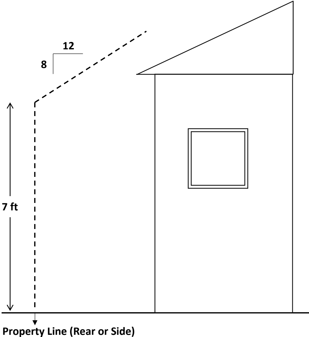
7-Foot, 8/12 Pitch Daylight Plane
