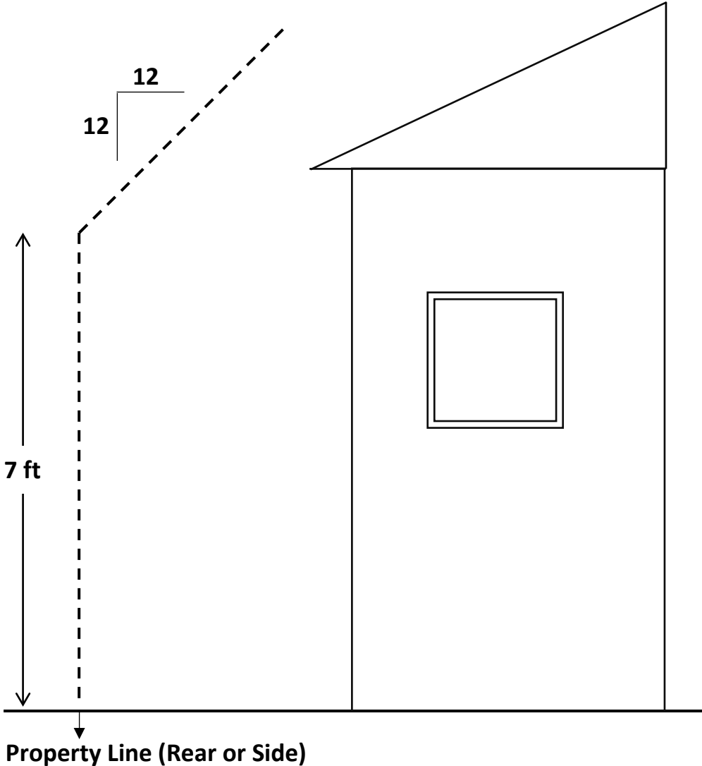
7-Foot, 12/12 Pitch Daylight Plane
