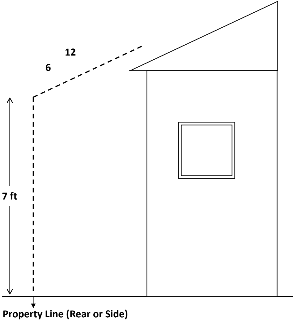
7-Foot, 6/12 Pitch Daylight Plane
