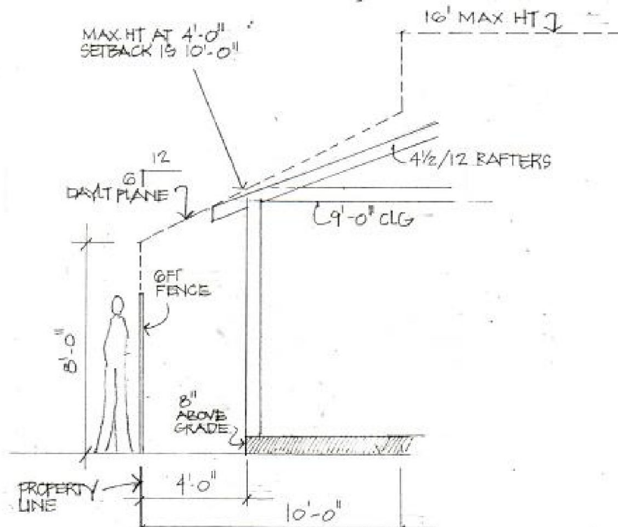
Figure 1-Standard Daylight Plane Diagram
