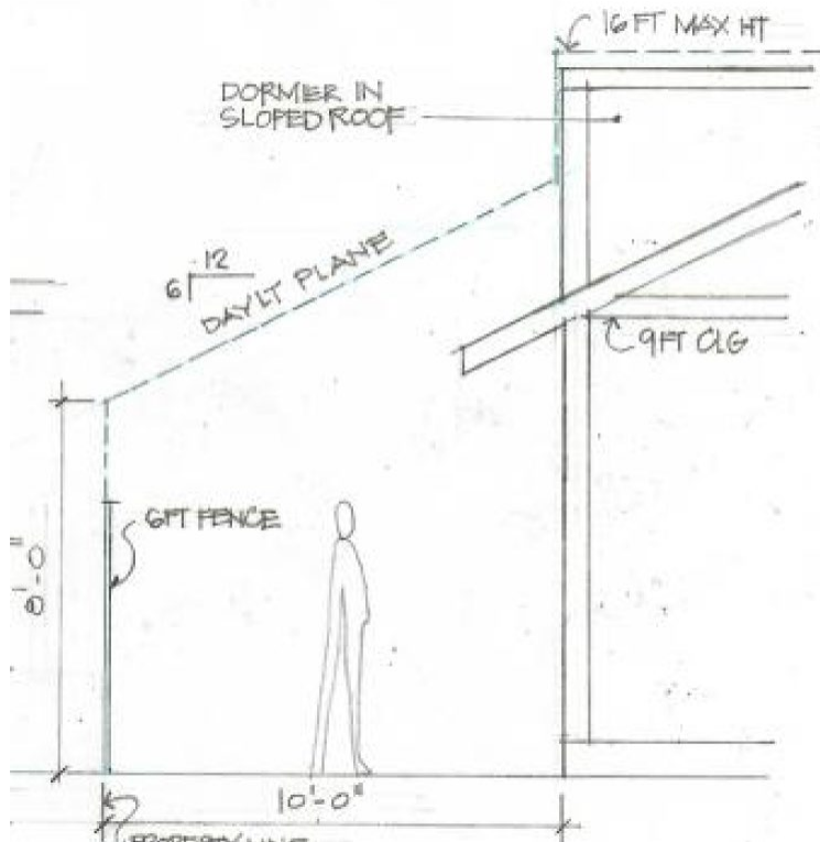
Figure 2-Voluntary Daylight Plane Diagram
