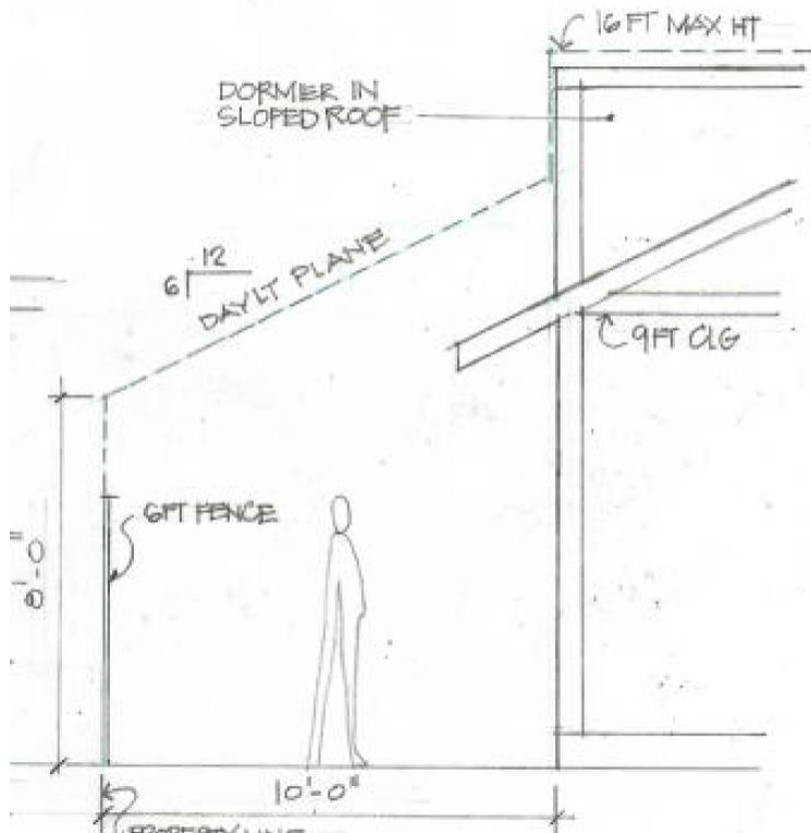
Figure 2-Voluntary Daylight Plane Diagram [A19]
