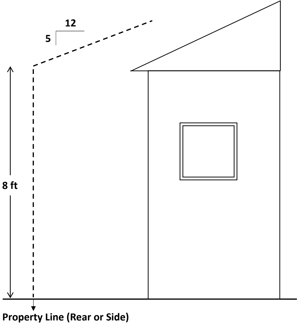
8-Foot, 5/12 Pitch Daylight Plane
