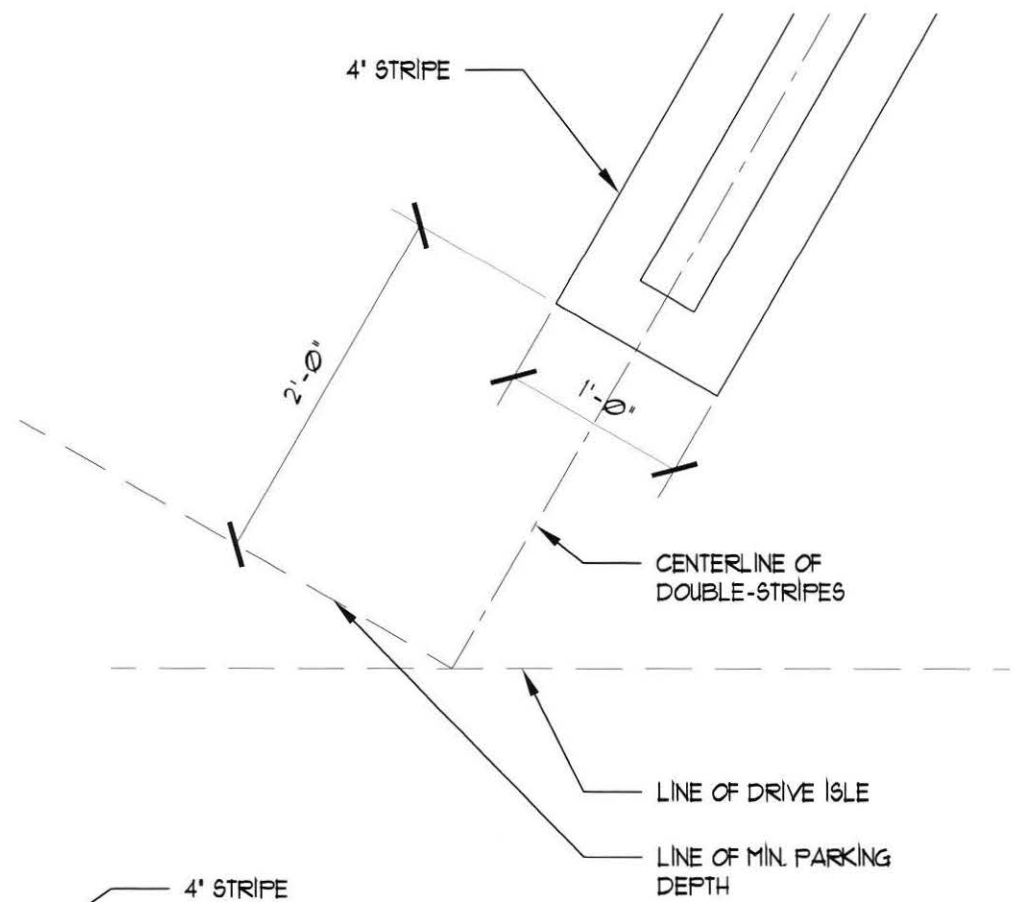
ANGLED STRIPING DETAILS SCALE: 1"=1'-0"
